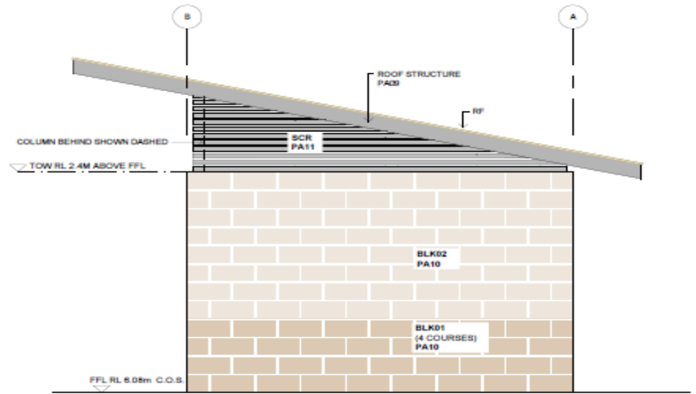
② STH / WEST ELEVATION 1:20
