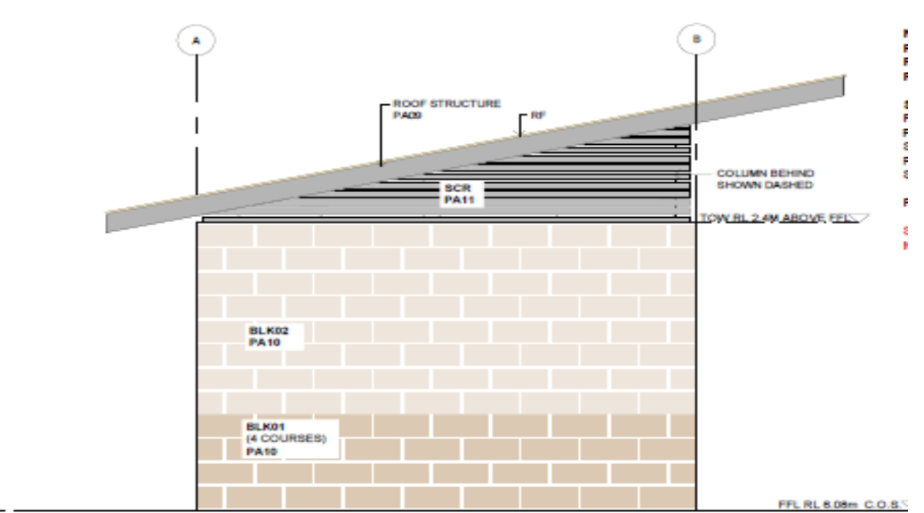
④ NTH / EAST ELEVATION 1:20
