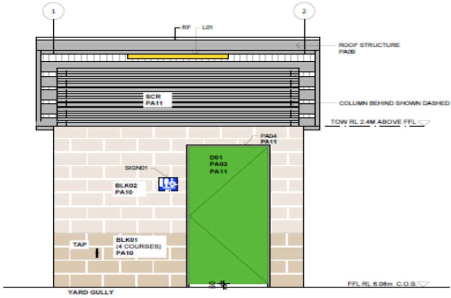
① NTH / WEST ELEVATION 1:20
