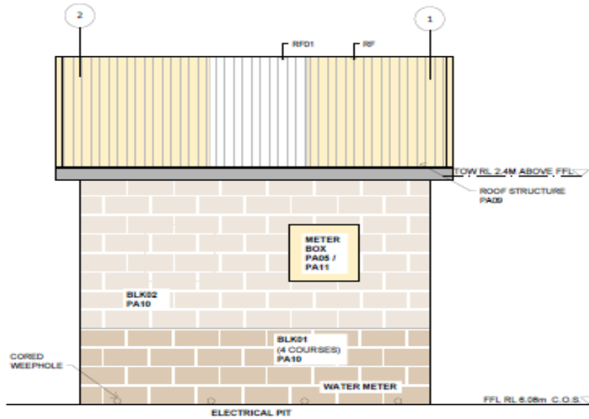
③ STH / EAST ELEVATION 1:20
