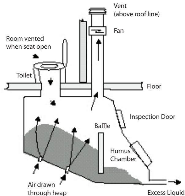
CROSS SECTION OF COMPOSTING
