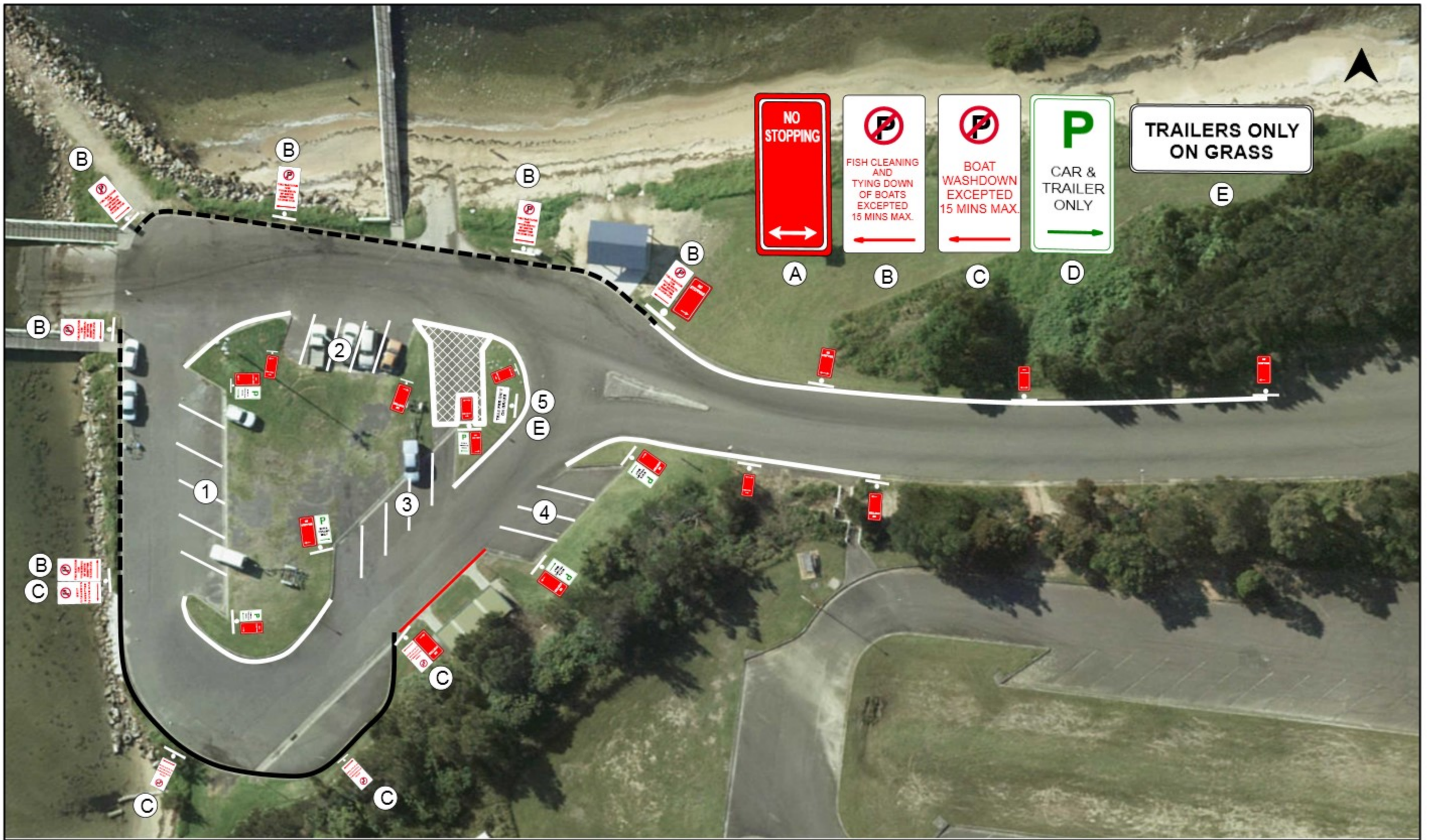
Proposed Parking restrictions, Signs and Line Marking Crookhaven Boat Ramp Car Park, Culburra Beach
