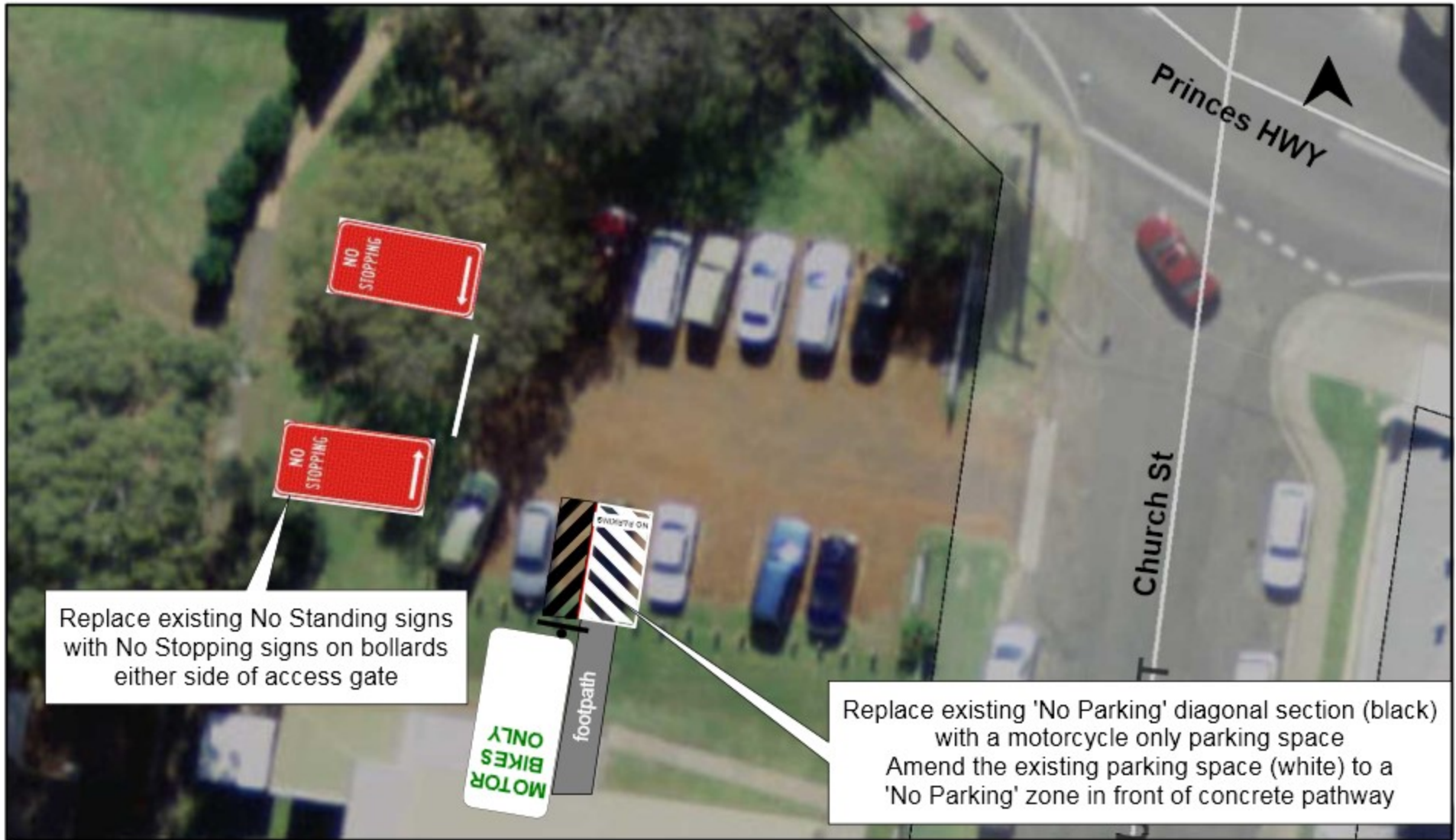
Proposed Signs and Line installation Milton Church Carpark, Milton
