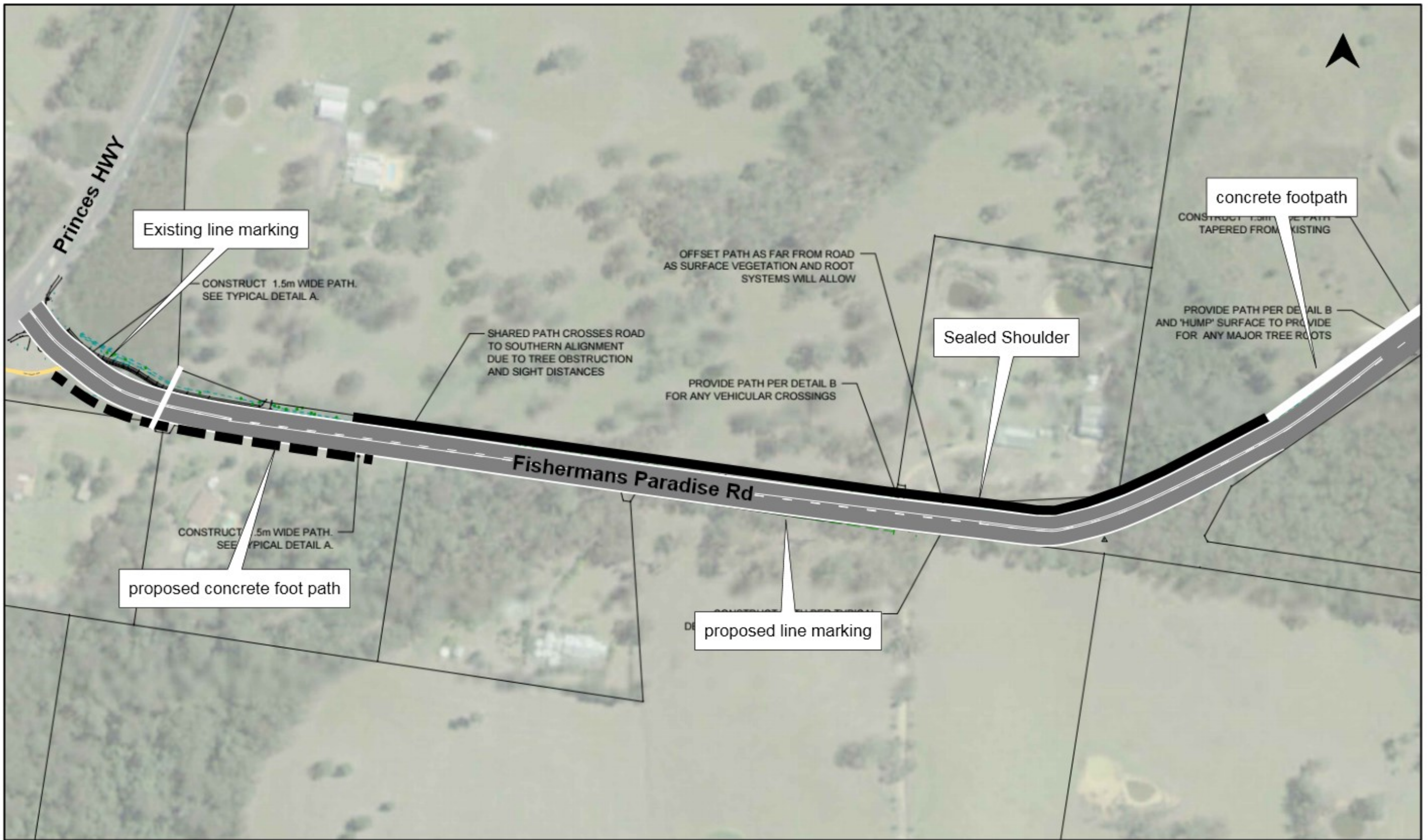
Proposed edge and centre line marking Fishermans Paradise Road, Fishermans Paradise
