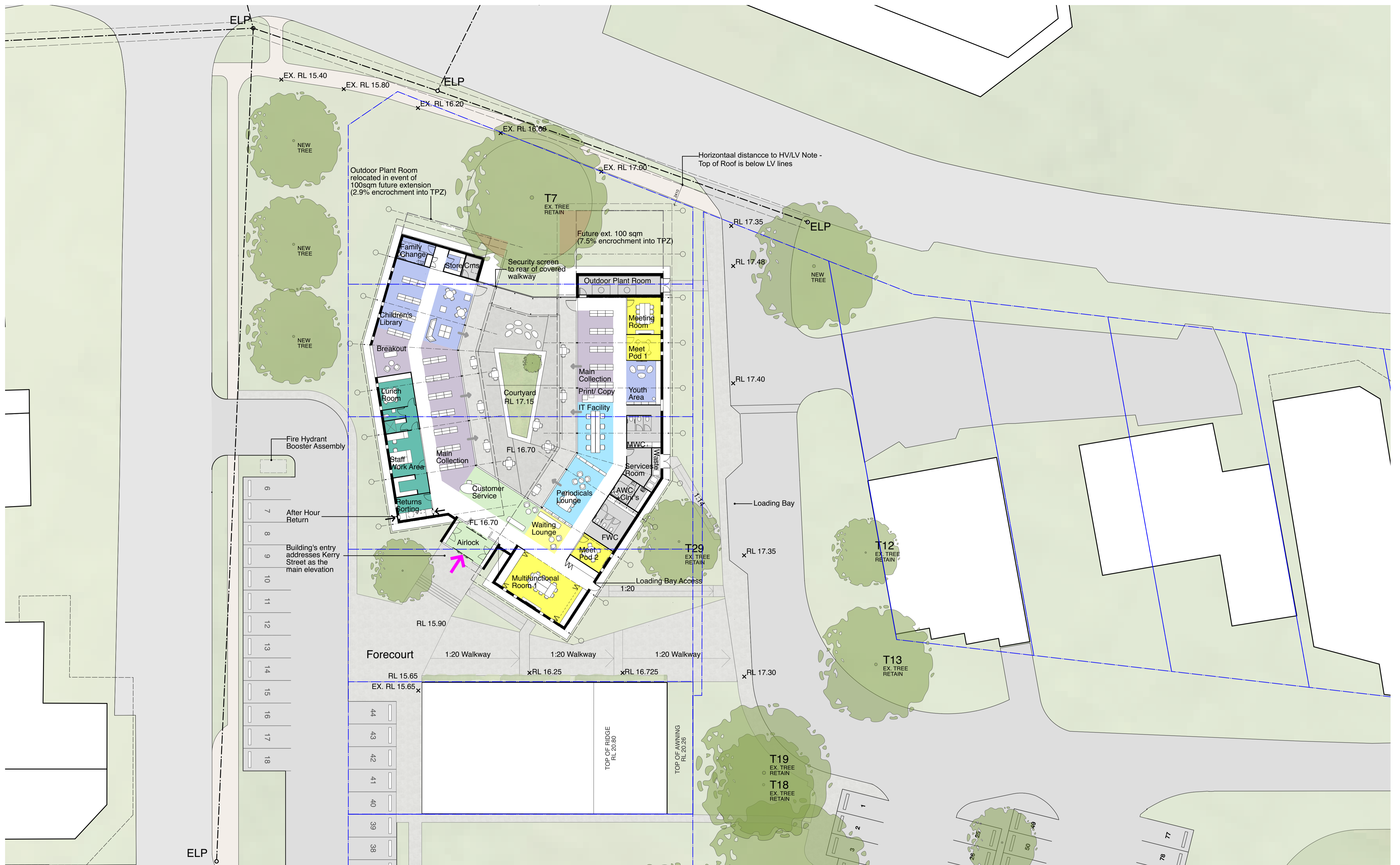
Floor Plan | Scale 1 : 200@A1
