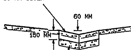
ELEVATION TYPE 2
