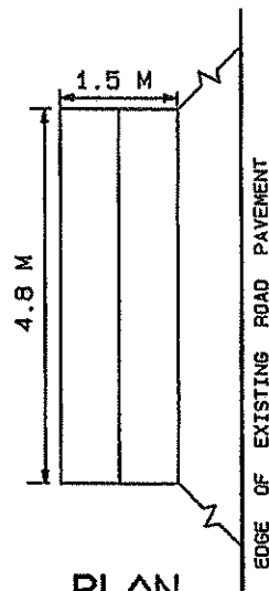
PLAN TYPE 2
