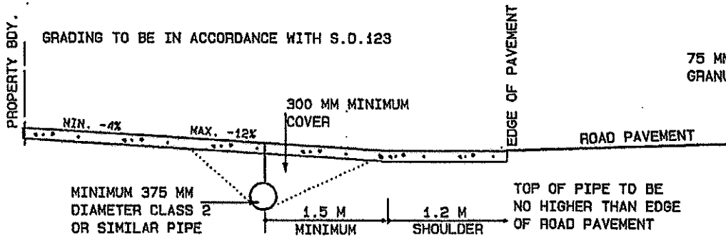
ELEVATION TYPE 1
