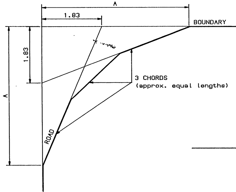
SQUARE JUNCTION
