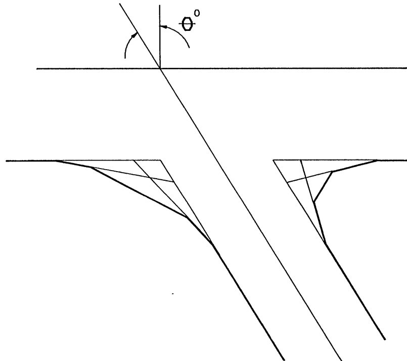
SKEW JUNCTION
