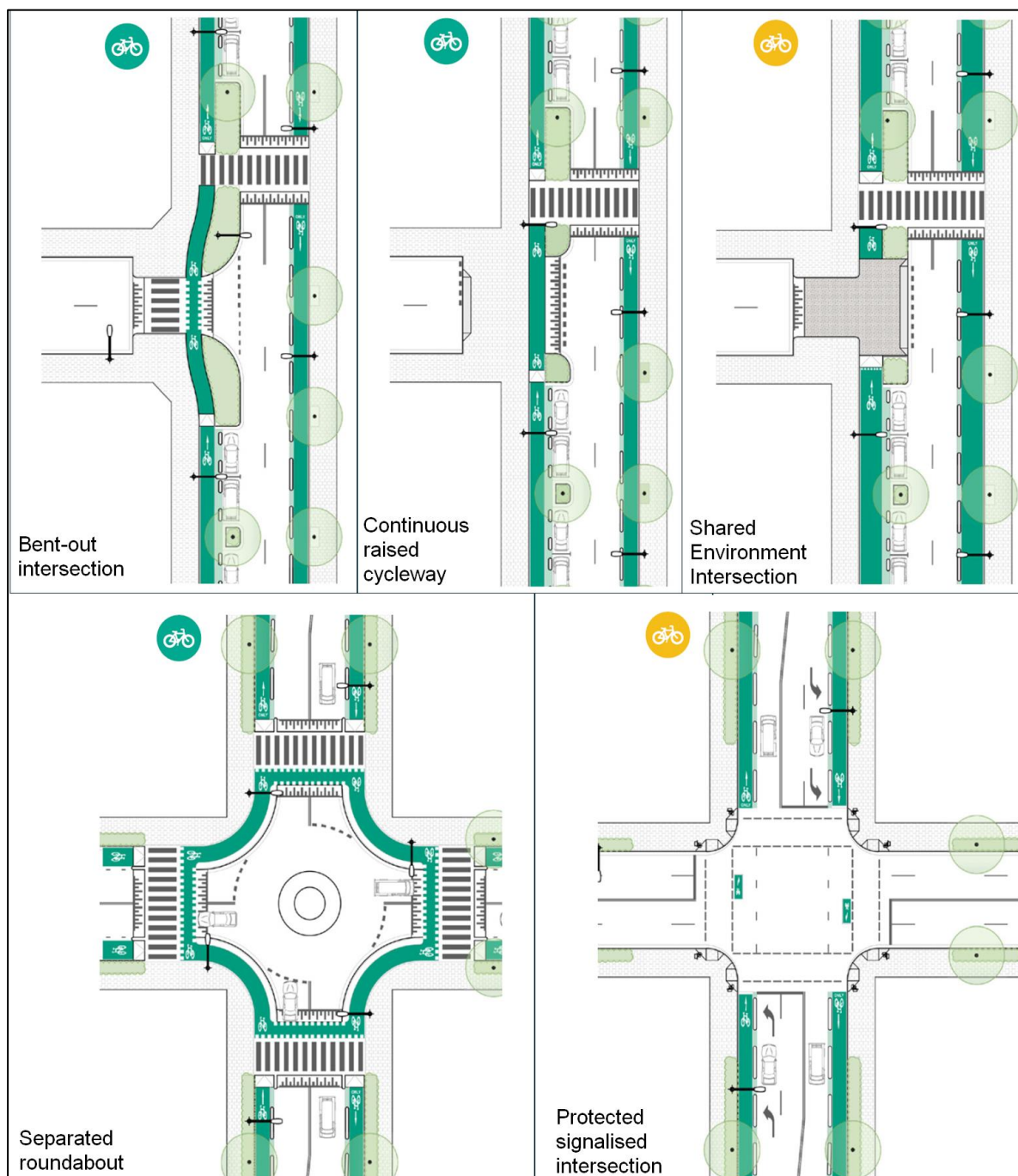
Figure 34: One-Way Bicycle Path Intersection Treatments
