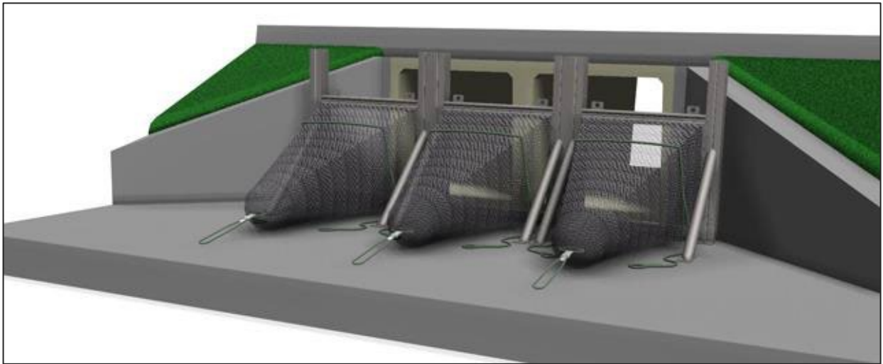
Figure C-15 Netted Trash Rack System Schematic (Urban Asset Solutions Pty Ltd, 2022)
