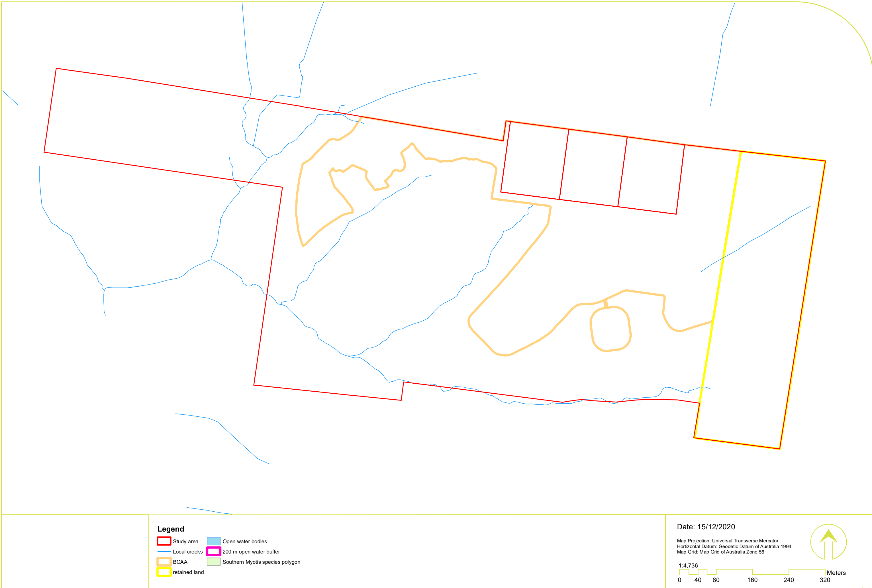
Figure 3-10: Southern Myotis habitat (habitat within 200m of open water)
