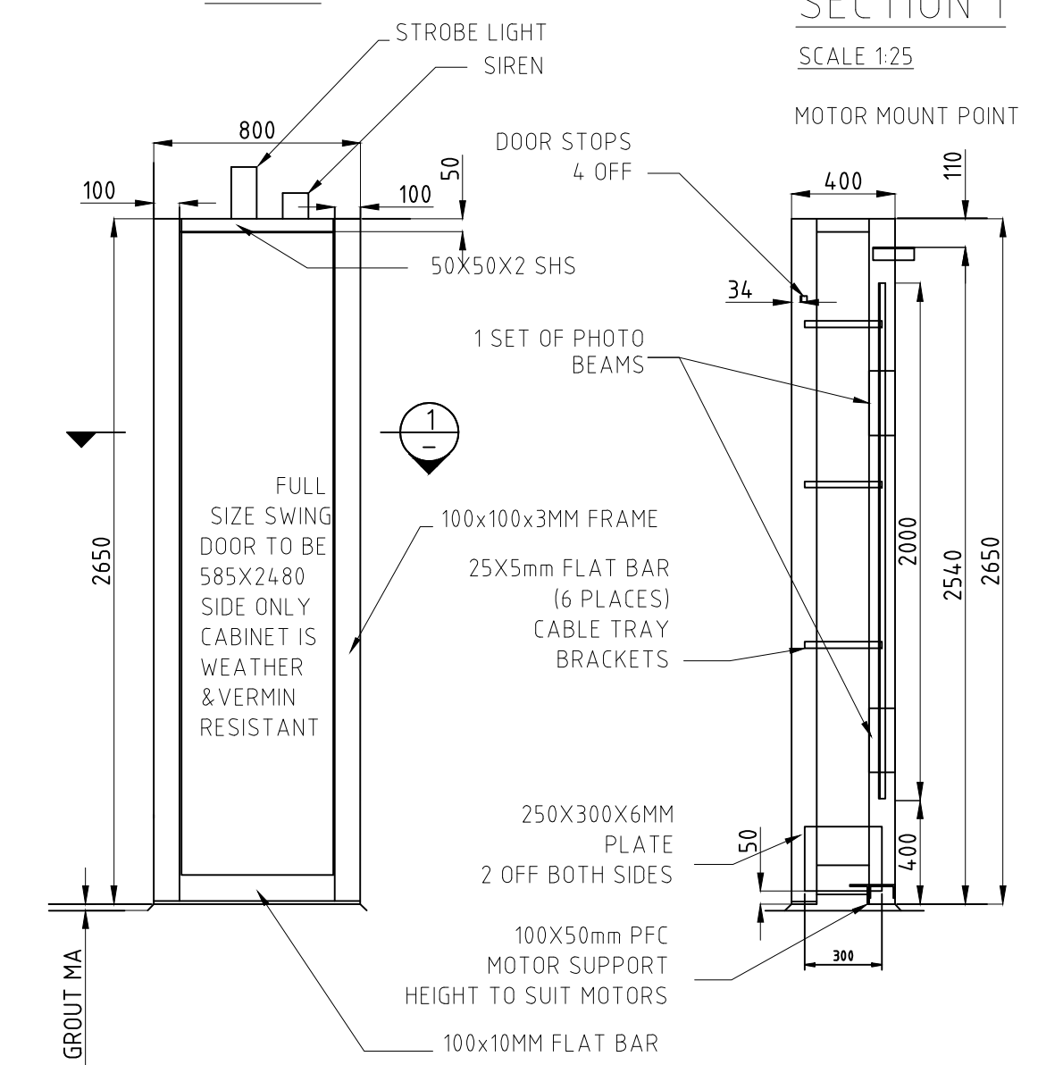
ELEVATION SCALE 1:25
