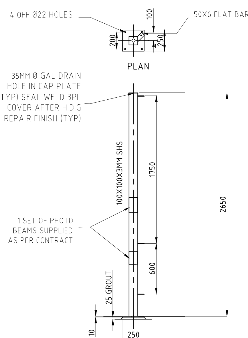
FENCE POST SCALE 1:25
