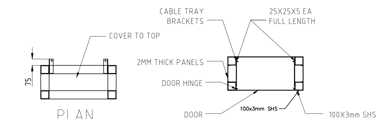
SECTION 1 SCALE 1:25
