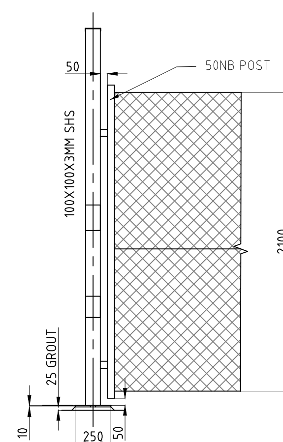
CONNECTION DETAIL WITH CHAINWIRE FENCE SCALE 1:25
