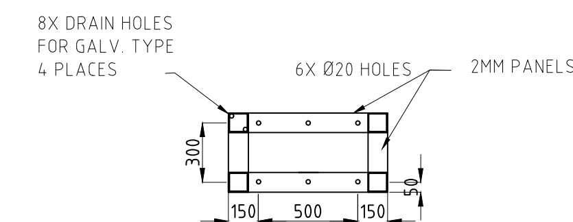
BOTTOM PLAN SCALE 1:25
