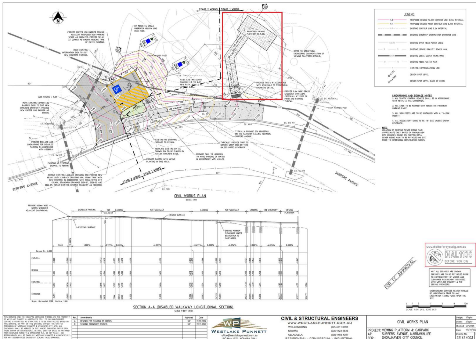
Figure 1 - Civil drawing extract of plans, construction of stage one works highlighted (red box).
