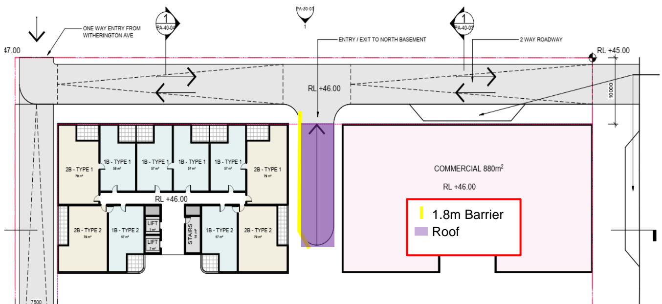
Figure 9-1 Carpark Ramp Treatment
