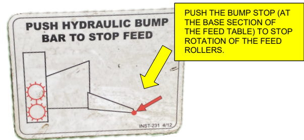
Fig1: PUSHING THE BUMP STOP
